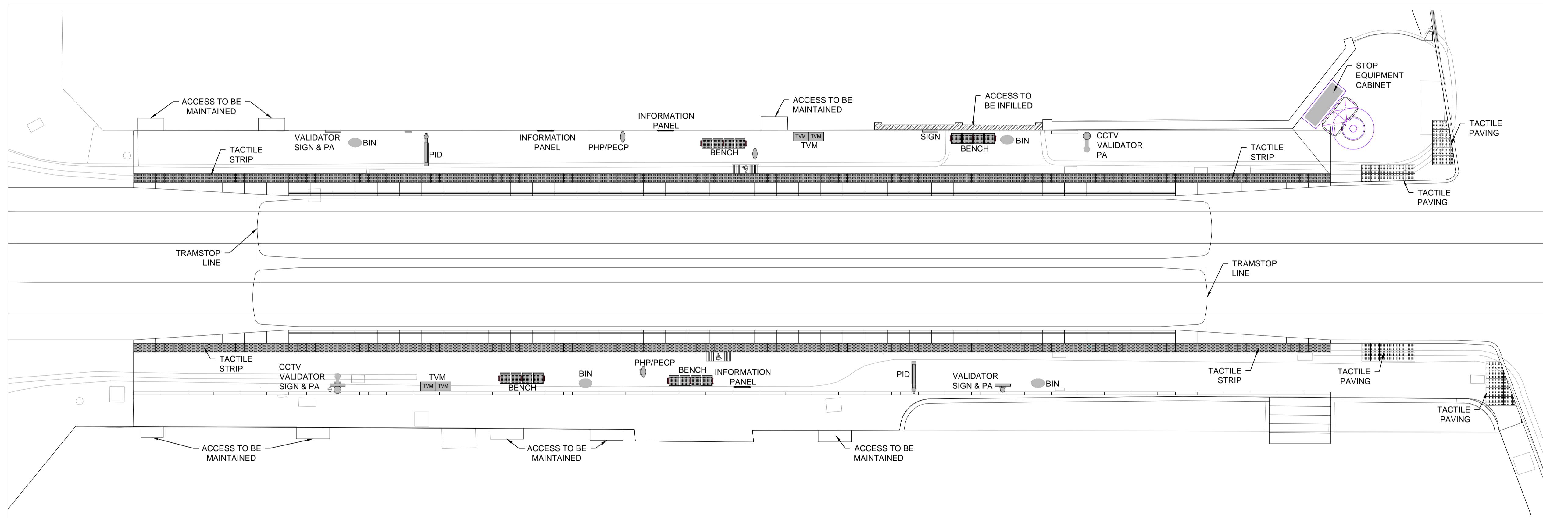
PROPOSED PLATFORM LAYOUT SCALE : N.T.S.
